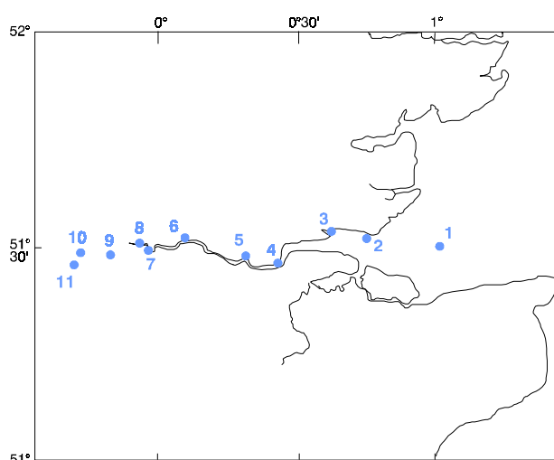
Figure 10. Thames transect
