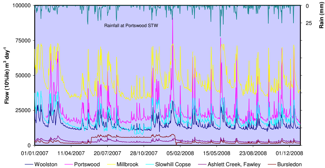
Figure 4.2: Flows for STWs discharging to Southampton Water, 2007-2008 (STW flow data provided by Southern Water, rainfall data provided by the Environment Agency).
