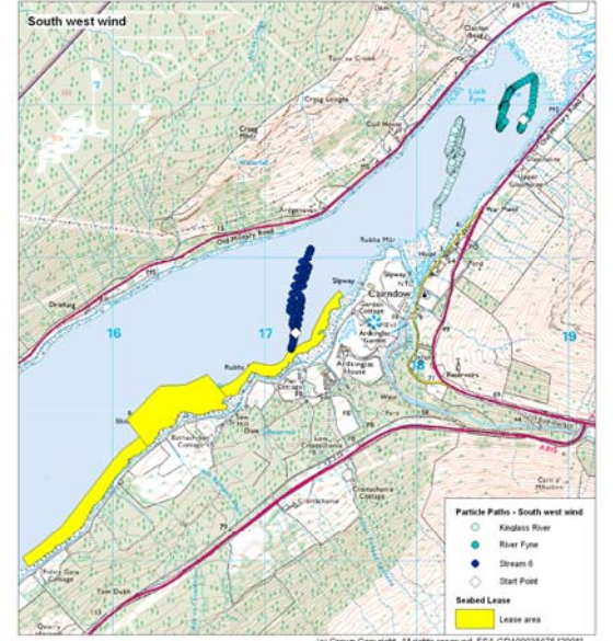
Figure 13.5 Cairndow, wind + tide particle paths from sources identified in the shoreline survey. The white diamond shows the start location.
