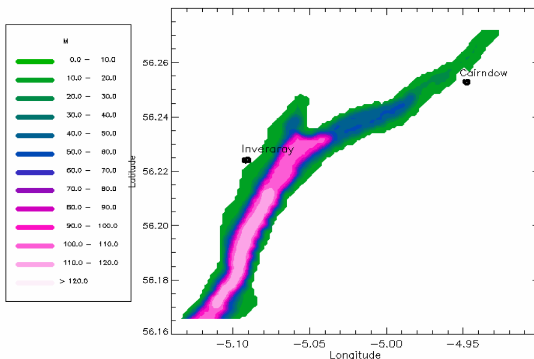
Figure 13.2 Model domain with depths (m).
