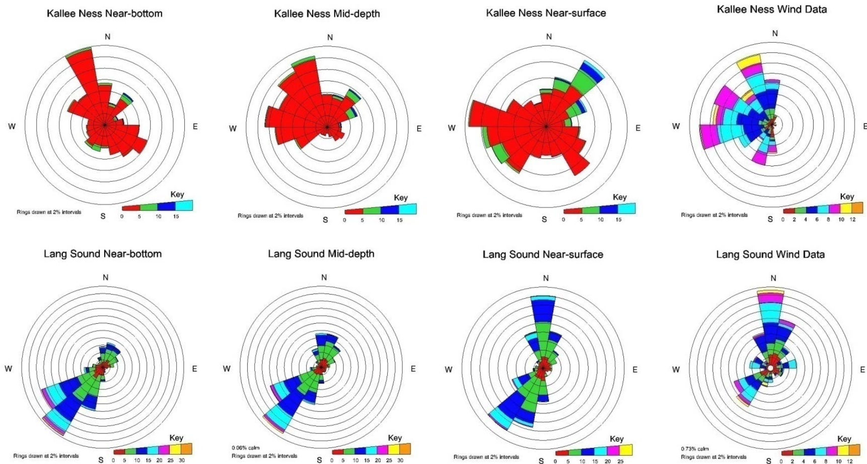
Figure 14.5 Current and wind plots for the Kallee Ness and Lang Sound fish farm surveys
