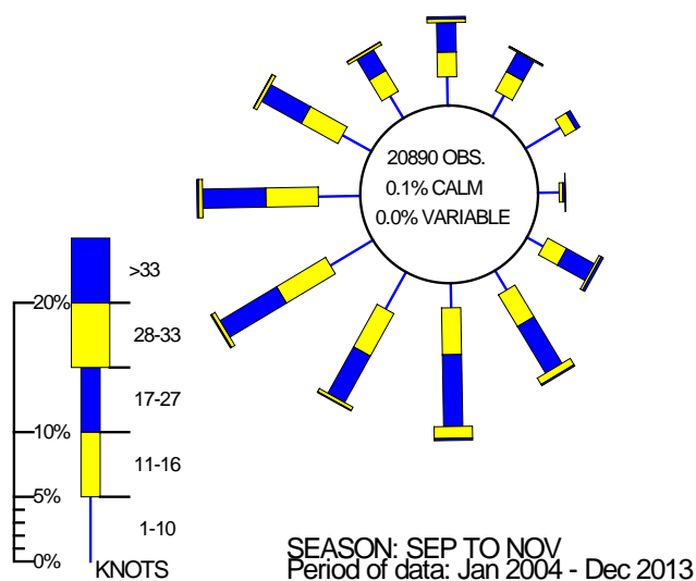
Figure 6.3 Seasonal wind roses for Tiree (2004-2013)
